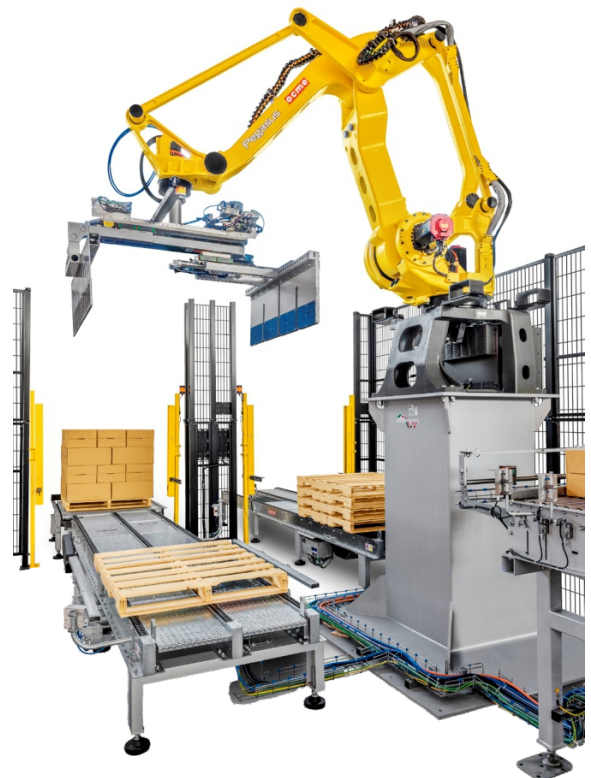
Robotic Palletizer
